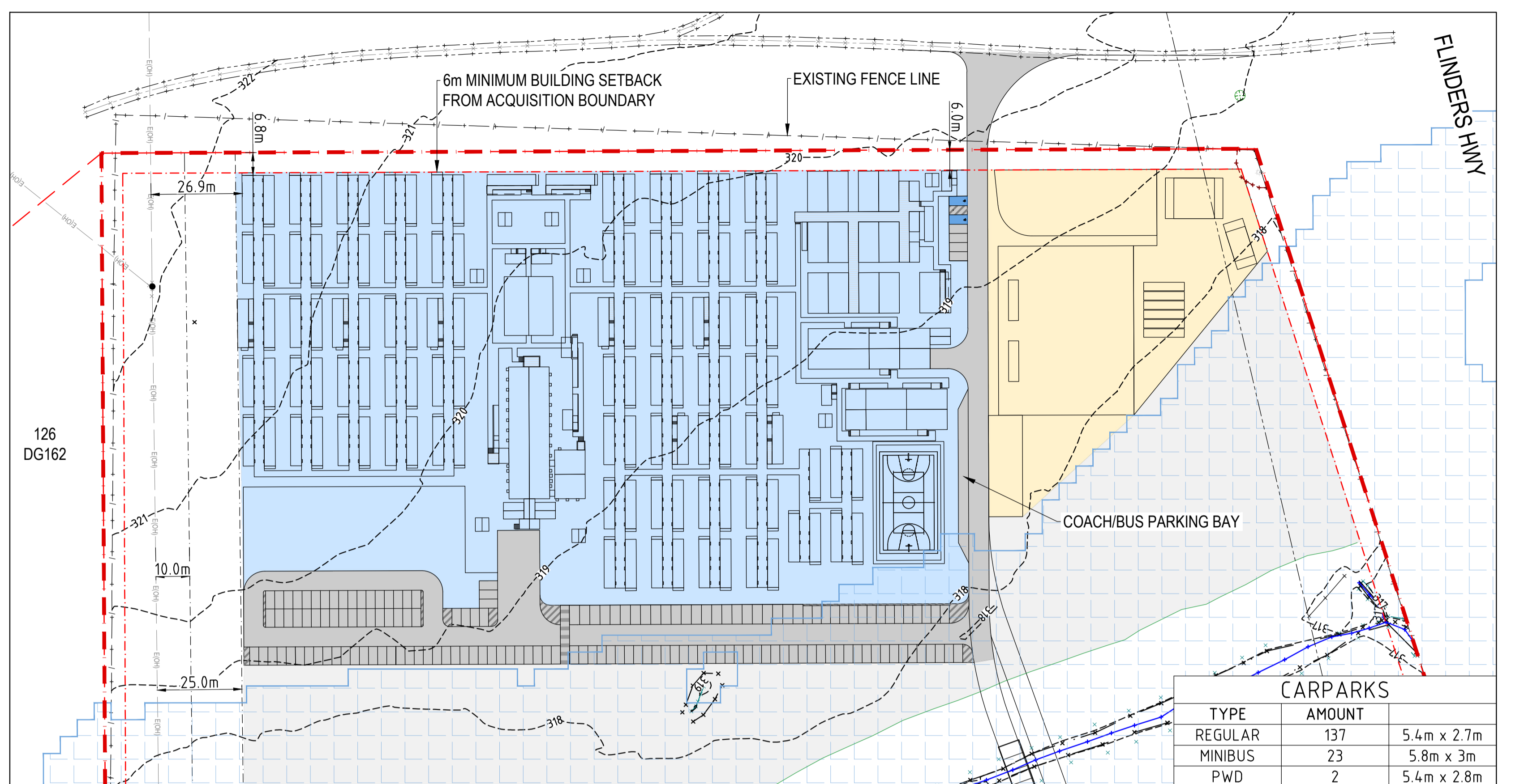
INSET - 410 PERSON CAMP SCALE 1:1000 (m)
