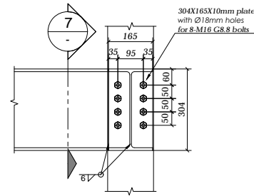
SECTION 5-5
