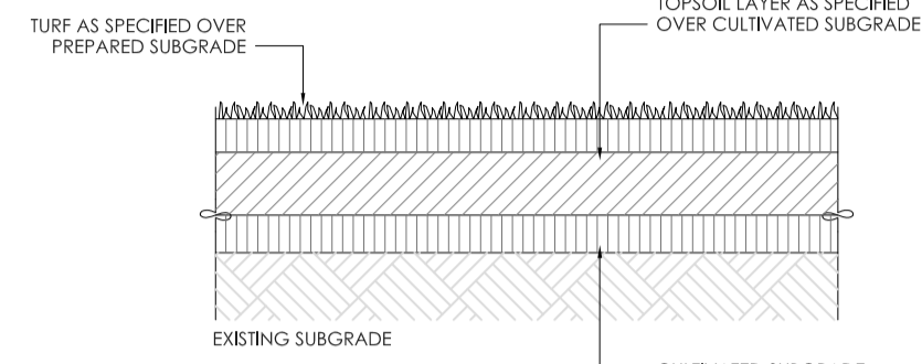
LD02 TURF DETAIL SCALE NTS
