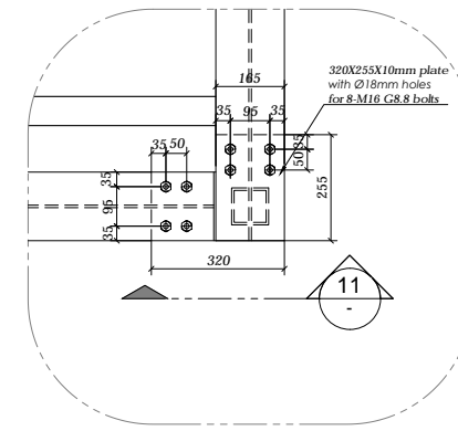
DETAIL-4
