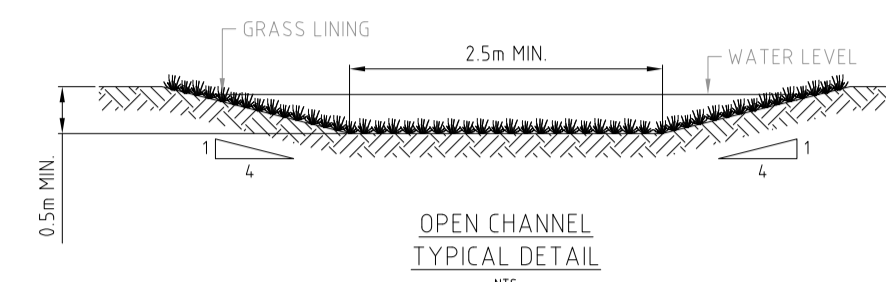
LD03 TURF SWALE DETAIL SCALE NTS (TYPICAL) DETAIL BY OTHERS
