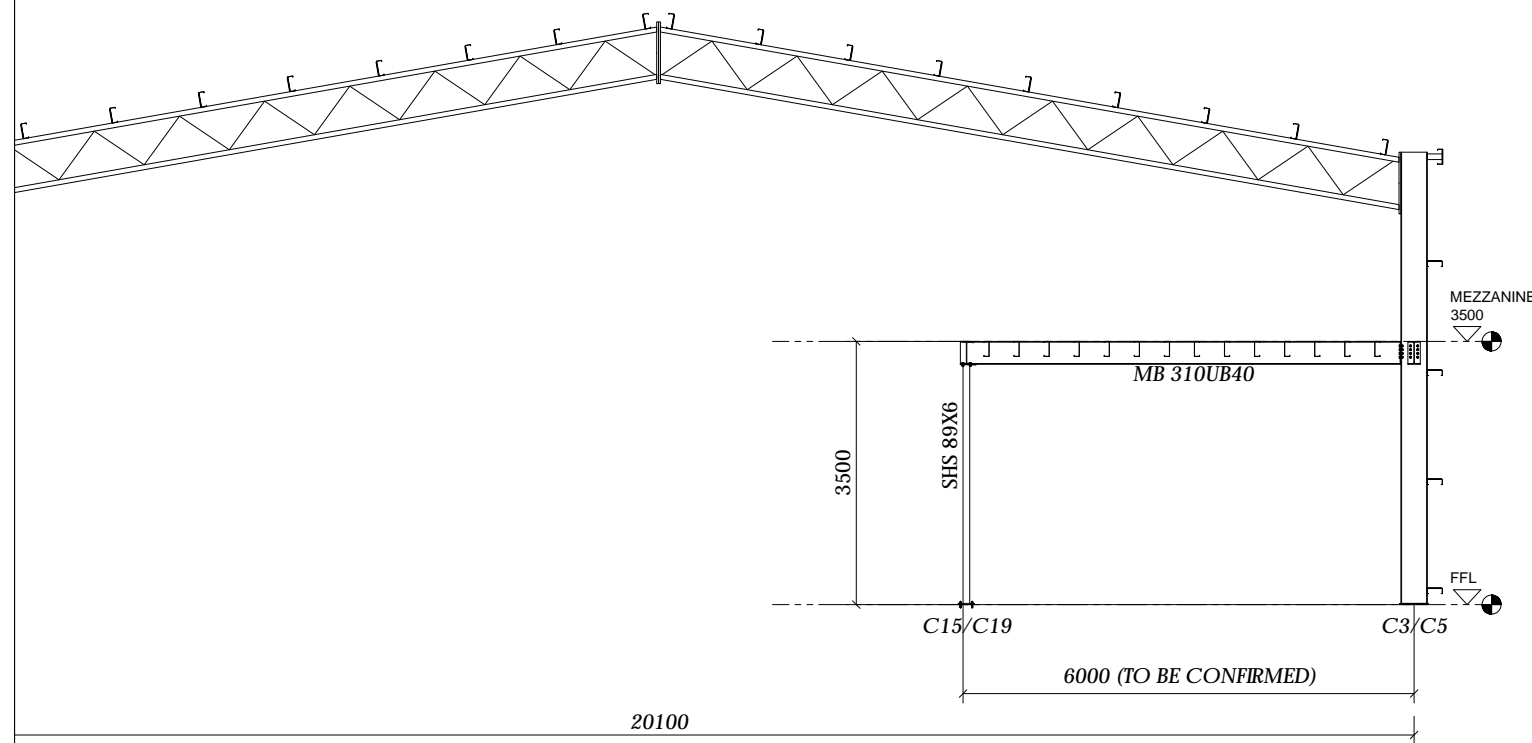
SECTION 3-3
