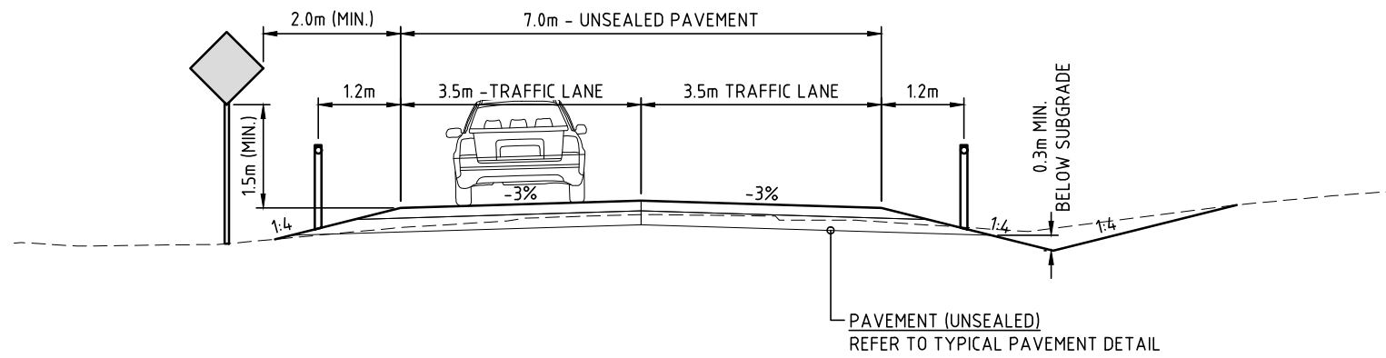
TYPICAL CROSS SECTION - INTERNAL ACCESS ROADS
