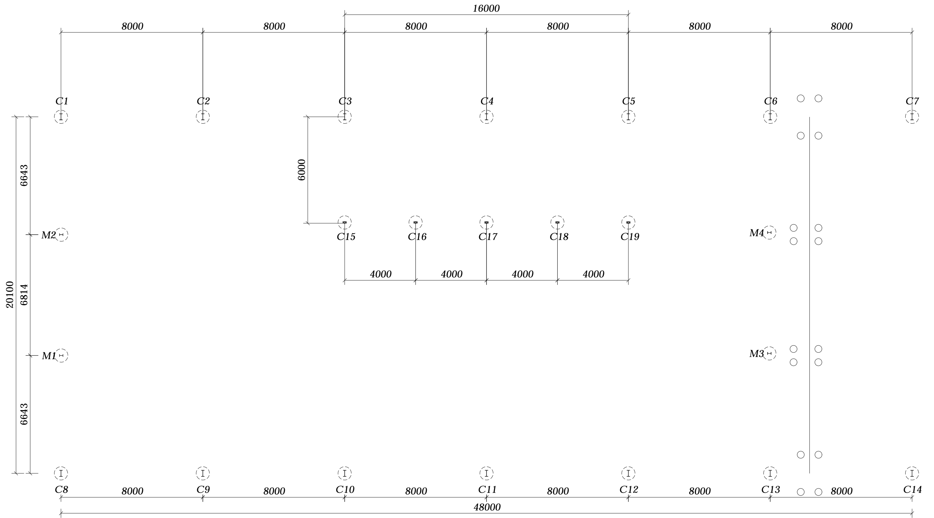
MEZZANINE FLOOR PLAN
