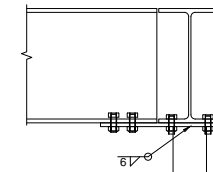
SECTION 11-11
