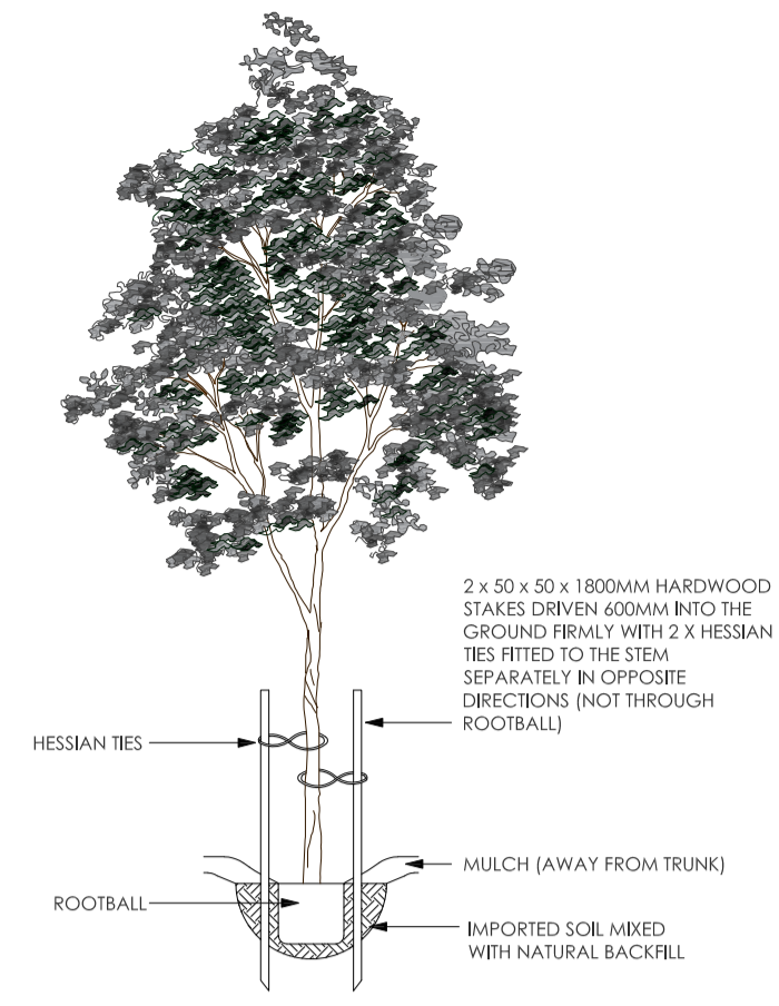
LD01 TREE PLANTING/STAKING DETAIL SCALE NTS (INDICATIVE)
