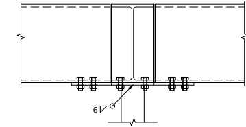
SECTION 13-13
